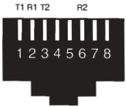
10 Base T
