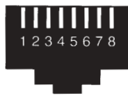
T568B, (AT&T) 8 position/8 wire
